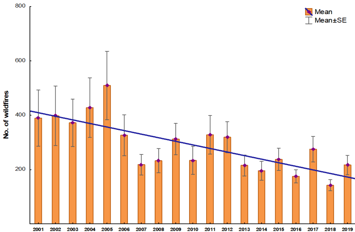
Figure 3. Mean yearly number of wildfires per province from 2001 to 2019. The blue line represents the regression fit of the mean values ( y = 422.5857 - 13.1319x ).
